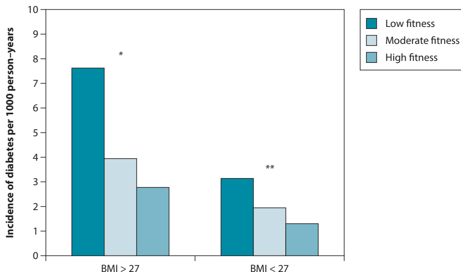
Figure 3.5 Metabolic fitness versus body weight and the incidence of diabetes
