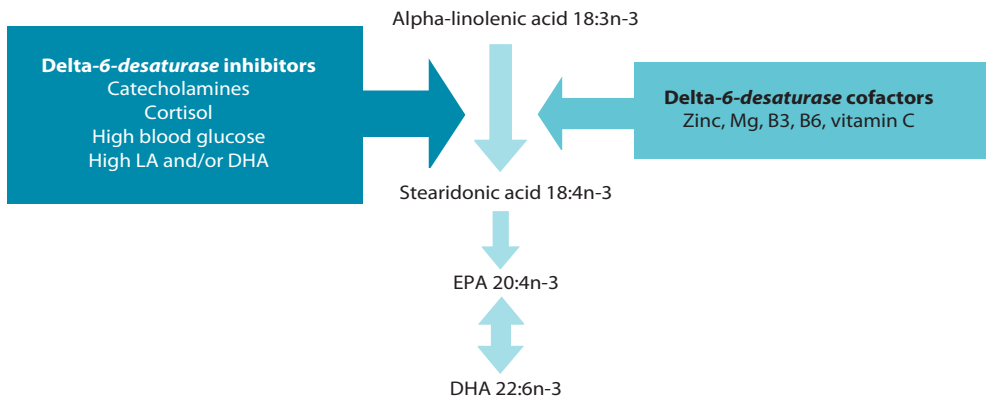
Figure 31.3 Enzyme modifiers of fatty acid conversion
