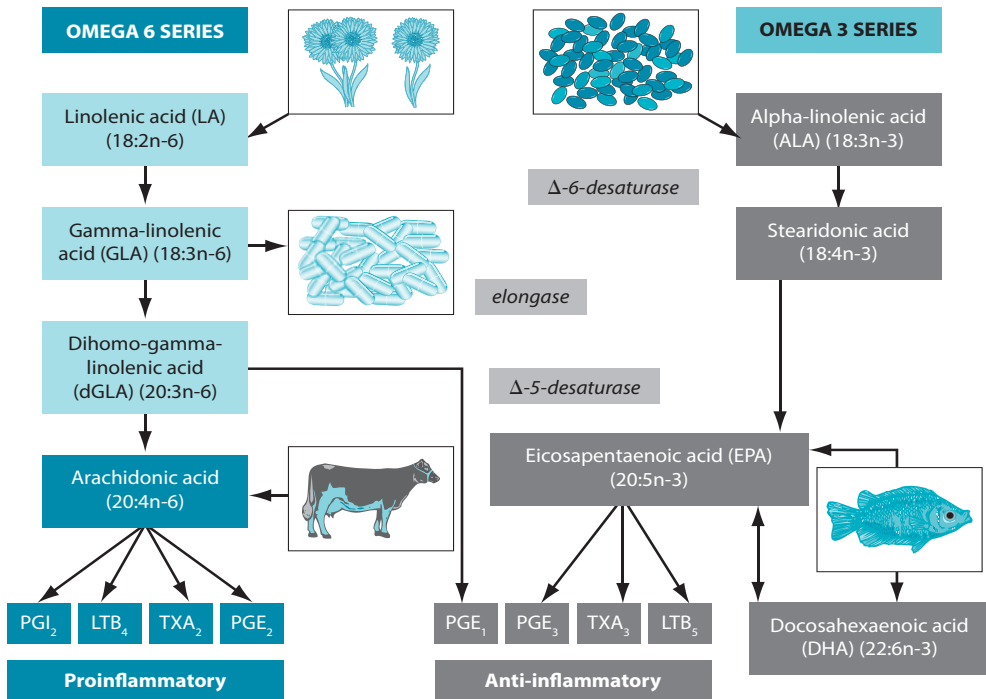
Figure 31.2 The metabolic pathways of essential fatty acids*
