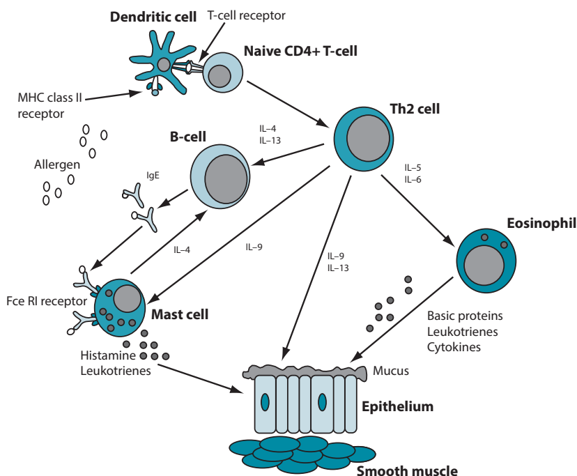
Figure 9.1 Mechanism of atopic asthma
