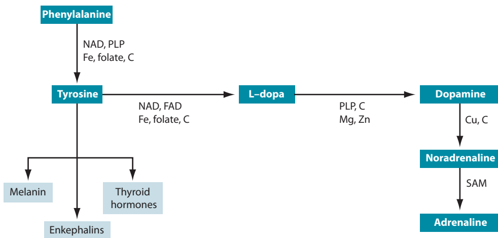
Figure 18.2 Catecholamine production
